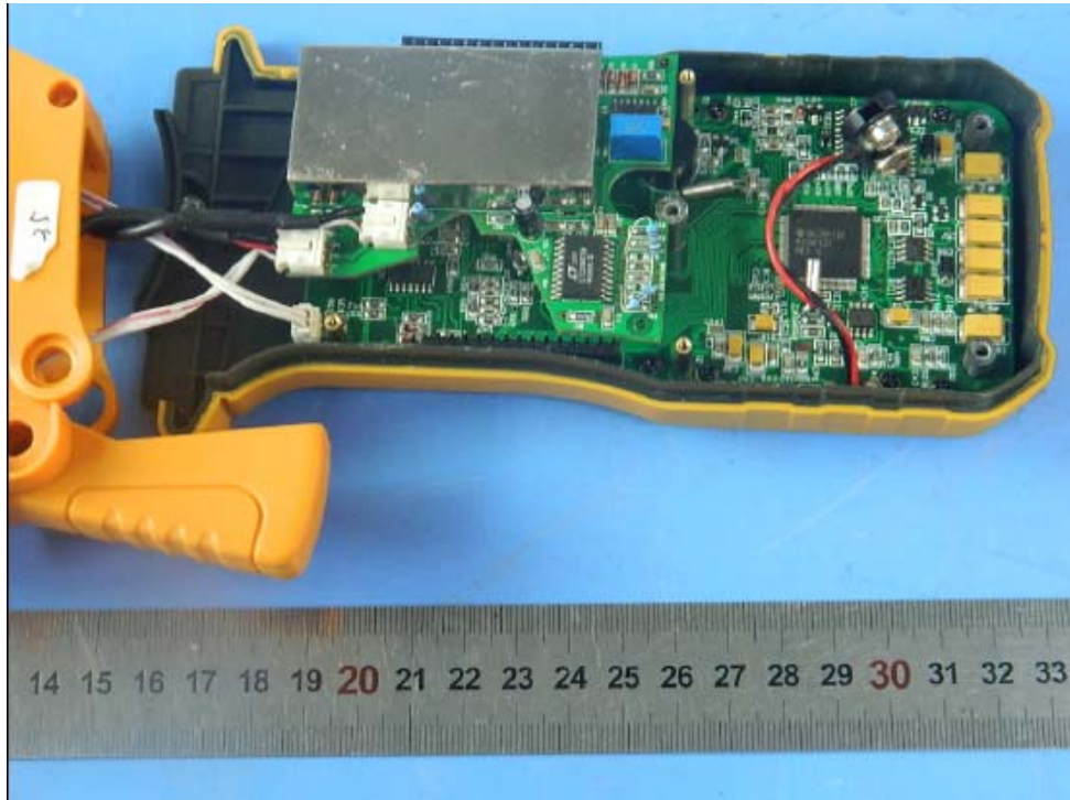
Photo 5# Unit internal view
