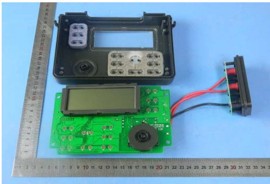
Photo 6# Internal View
