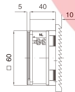
风扇及过滤器 Fan and filter JL9800.230
