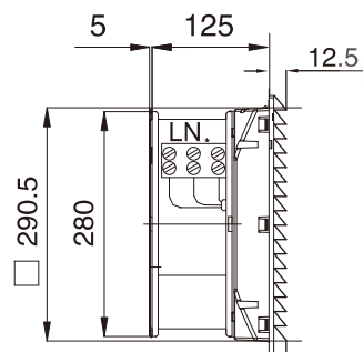
风扇及过滤器 Fan and filter JL600.230
