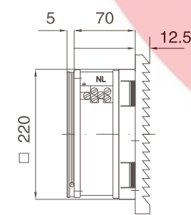
风扇及过滤器 Fan and filter JL9805.230
