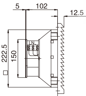
风扇及过滤器 Fan and filter JL400.230
