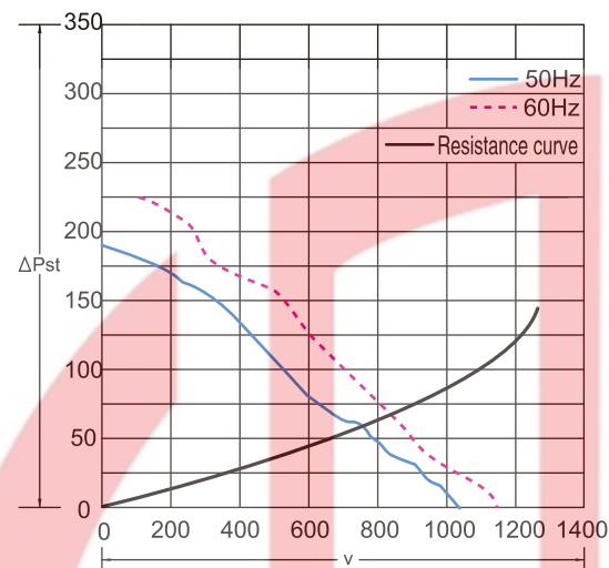
V=容积电流 Volume of current ( m 3 /h ) ΔPst=静止压差 Static pressure difference ( Pa )
