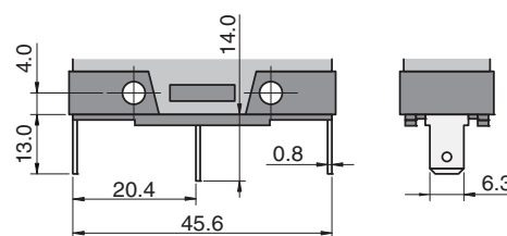
Terminal Faston (Quick Connect)
