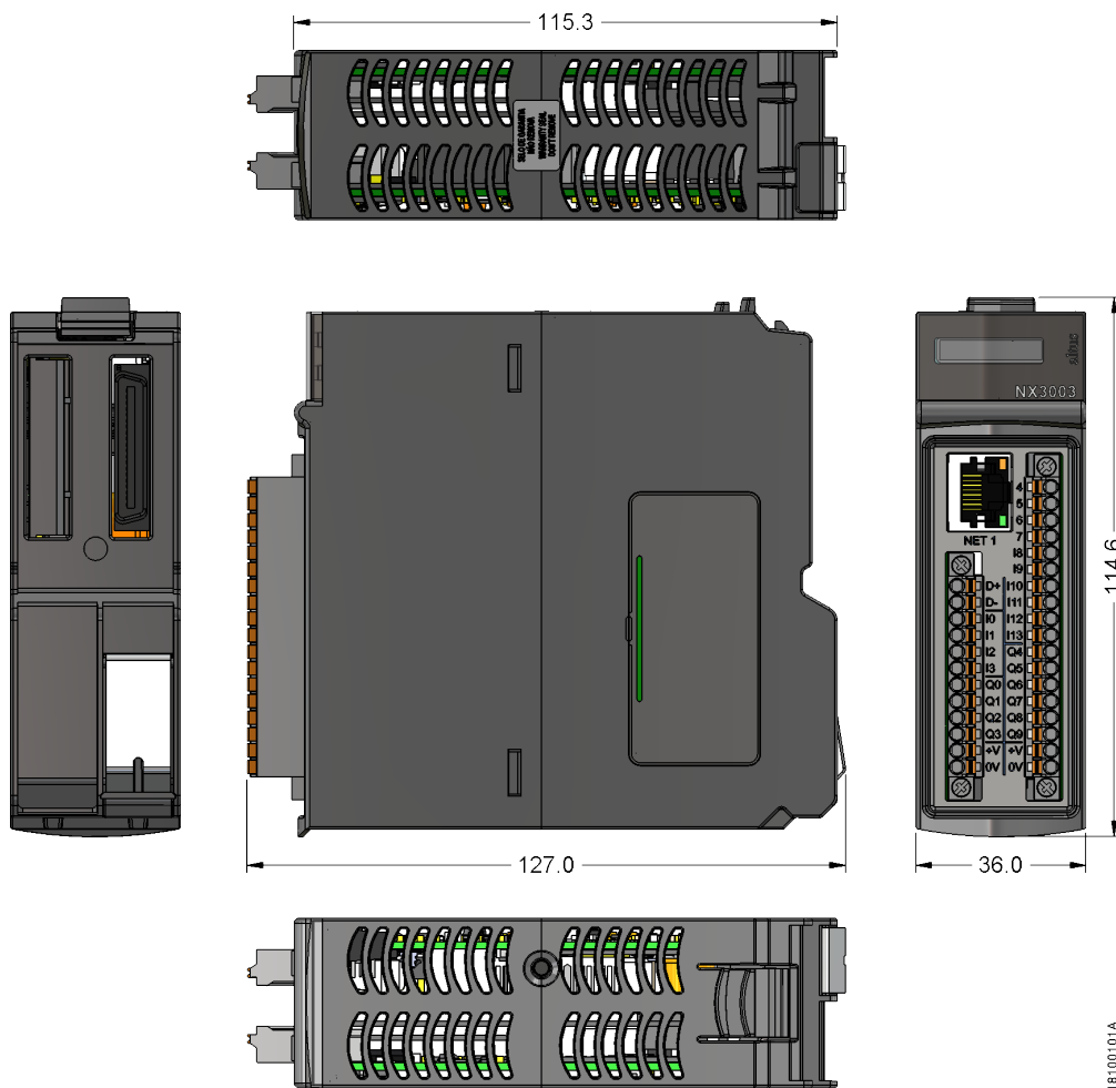
Figure 1: NX3003 CPU Physical Dimensions
