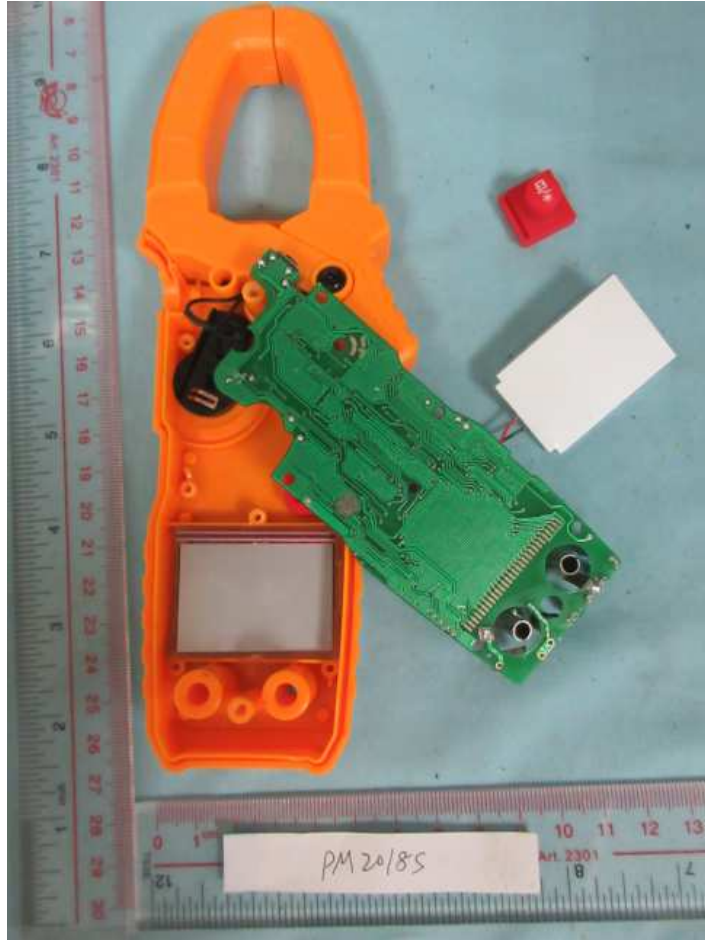
Photo 11: PCB bottom view of PM2018S
