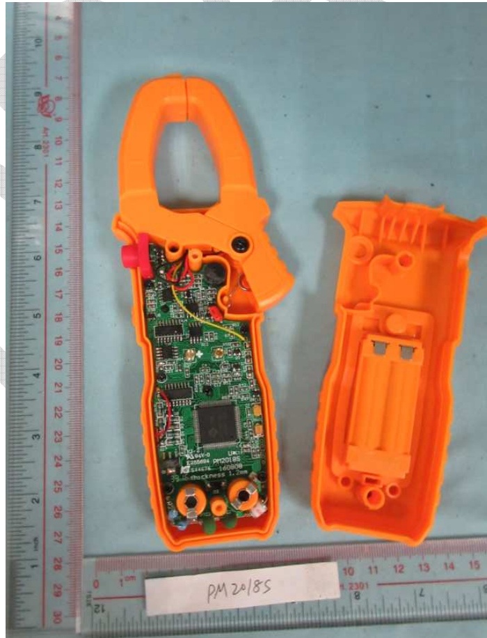
Photo 10: Internal view of PM2018S
