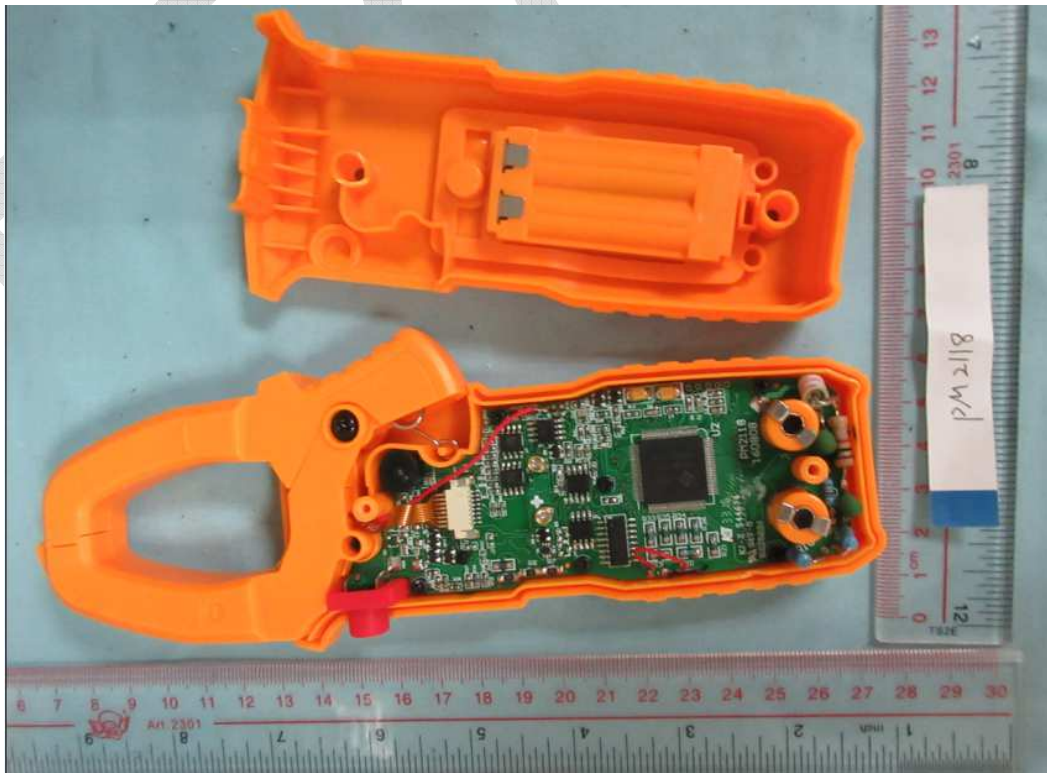
Photo 12: Internal view of PM2118
