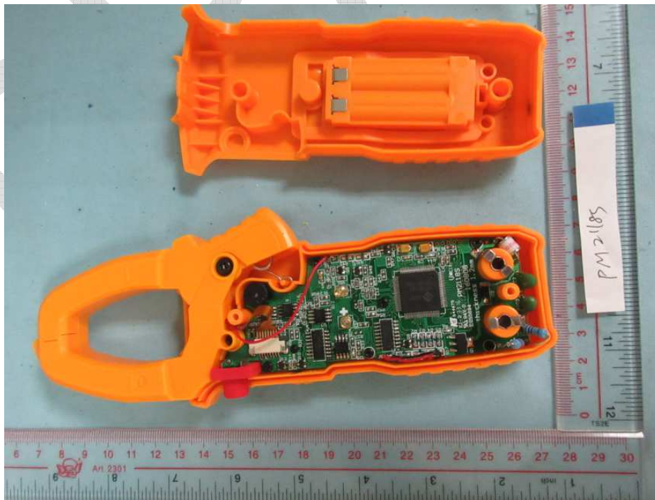
Photo 14: Internal view of PM2118S
