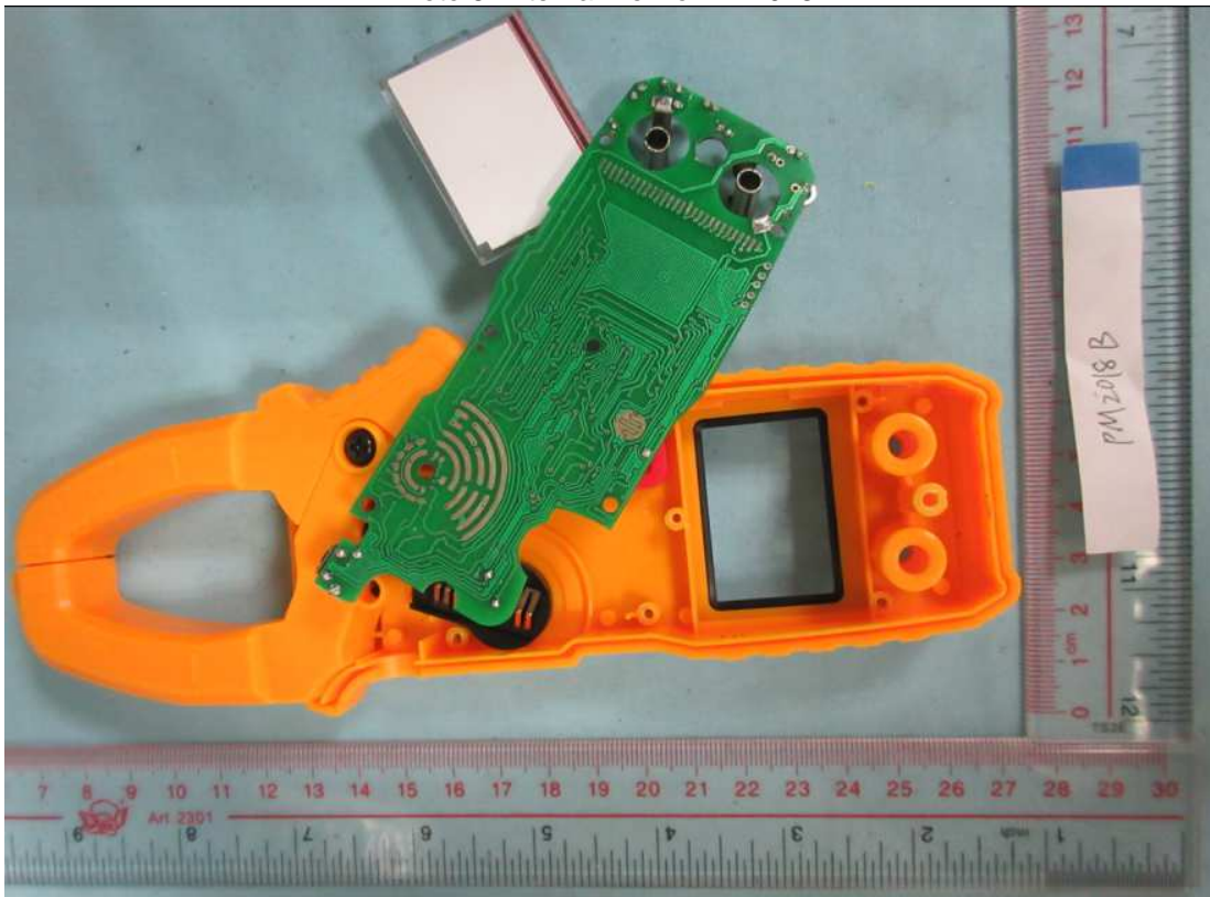
Photo 9: PCB bottom view of PM2018B
