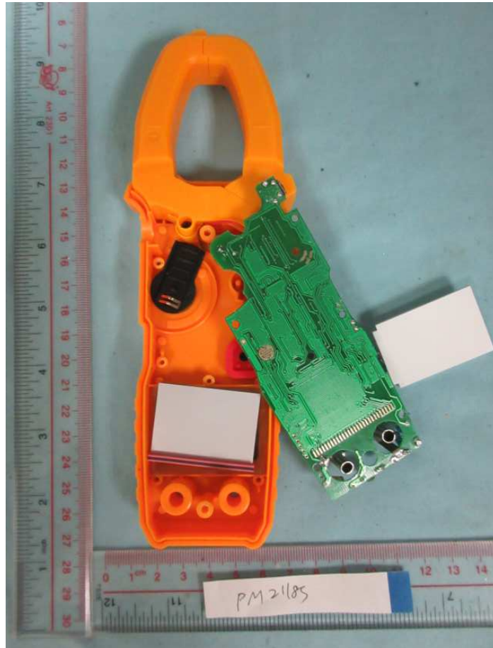
Photo 15: PCB bottom view of PM2118S
