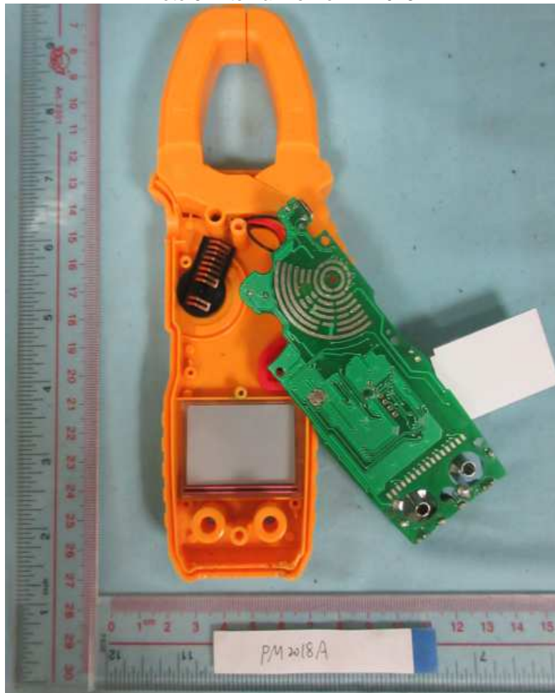
Photo 7: PCB bottom view of PM2018A
