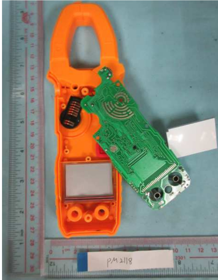
Photo 13: PCB bottom view of PM2118
