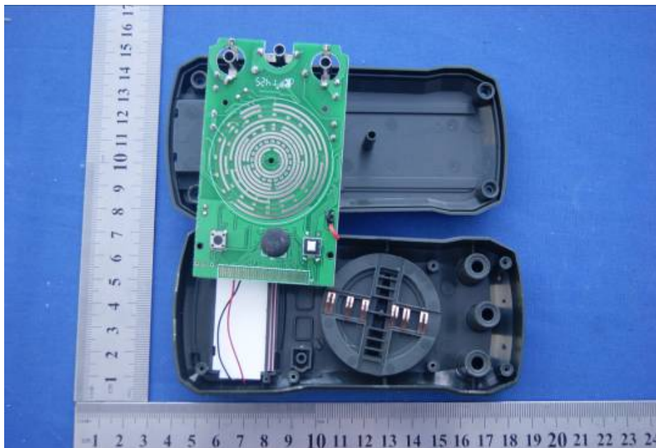
Photo 4# PCB on trace side
